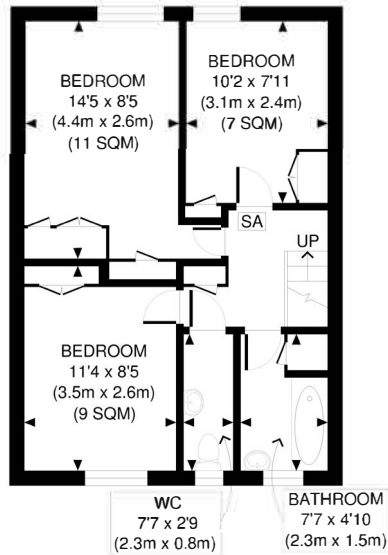
THIRD FLOOR GROSS INTERNAL FLOOR AREA 421 SQ FT
